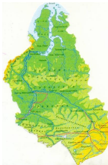
Fig. 1 – Physiographic map of Western Siberia [1]
